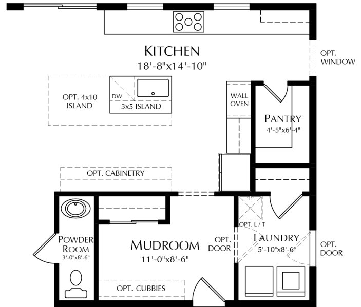
GOURMET KITCHEN + 91 SQFT ADDS 2' EXTENSION TO THE KITCHEN AND BREAKFAST NOOK OFF REAR, CHANGES THE KITCHEN LAYOUT TO INCLUDE A WALK-IN PANTRY, AND ADDS A 2' EXTENSION TO THE MUDROOM & LAUNDRY OFF FRONT.
